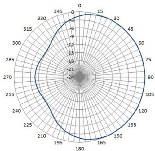
TYPICAL RADIATION PATTERN (HORIZONTAL PLANE)
