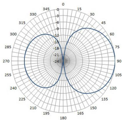
TYPICAL RADIATION PATTERN (VERTICAL PLANE)
